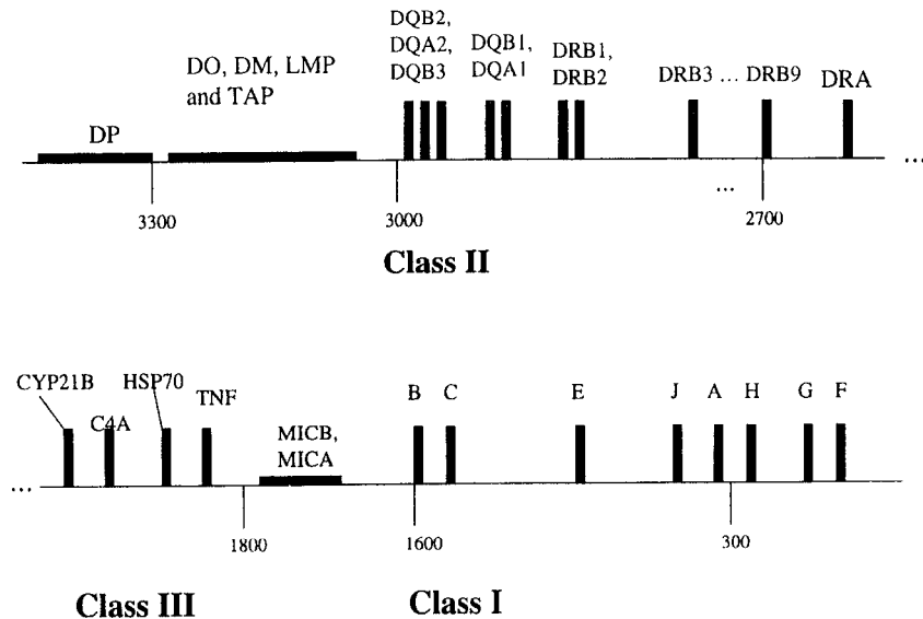
FIG. 1. Outline of the major histocompatibility complex region on chromosome 6.
